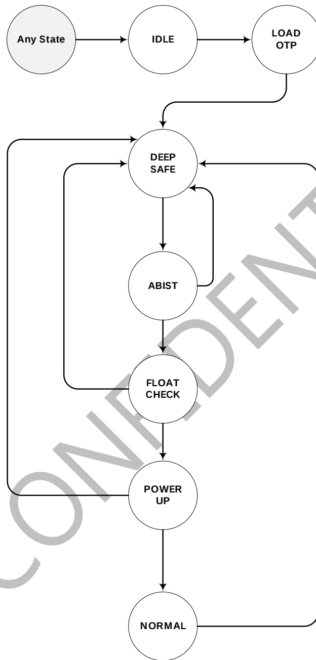
Figure 14. Operating State Machine and Transitions
