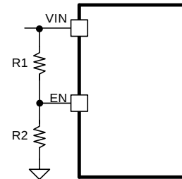
Figure 14. System UVLO by enable divide
